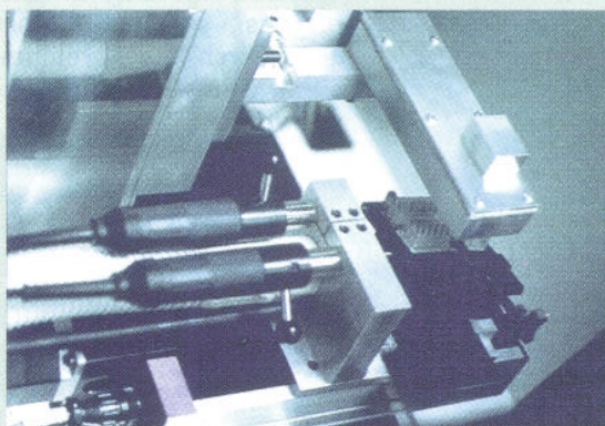
FIGURE 2 The PRO-CAM CAM station.
